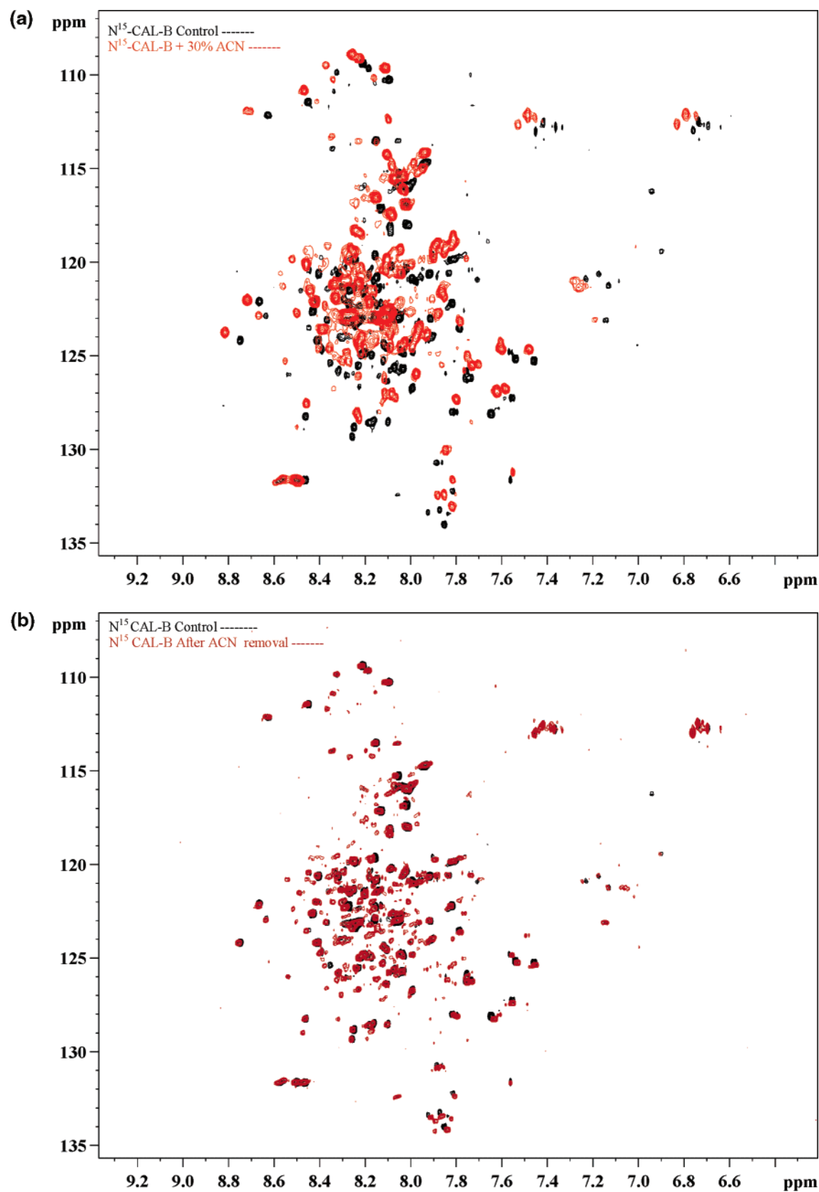
Figure 8. (a) 2D ^1\text{H}/^{15}\text{N} TROSY spectra. The \text{N}^{15} -CAL-B control spectrum is displayed in black, and the \text{N}^{15} -CAL-B containing 30% acetonitrile is shown in red. (b) 2D ^1\text{H}/^{15}\text{N} TROSY spectra. The \text{N}^{15} -CAL-B control spectrum is displayed in black, and the \text{N}^{15} -CAL-B after acetonitrile removal is shown in red.
